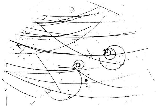
FIG. 1. A photograph of a typical double internal conversion.
